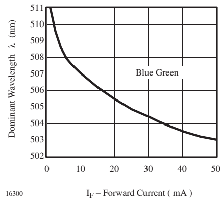
16300 Figure 34. Dominant Wavelength vs. Forward Current
