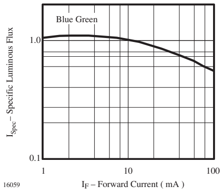
16059 Figure 31. Specific Luminous Flux vs. Forward Current
